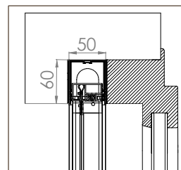
BORA TOP INCAS STANDARD 50/20
