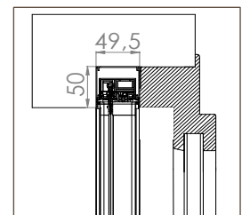
BORA TOP INCAS MIDI 50/20
