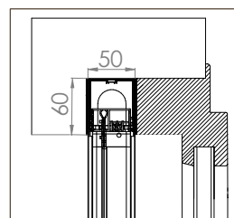
BORA TOP INCAS STANDARD 50/50
