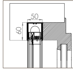
BORA TOP INCAS SR STANDARD 20
