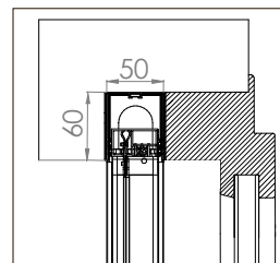
BORA TOP INCAS STANDARD 35/35
