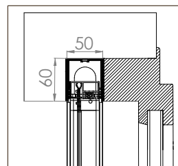
BORA TOP INCAS STANDARD 50/35
