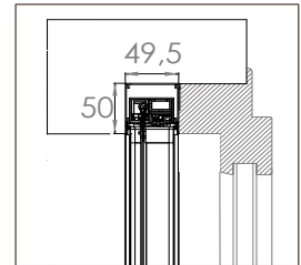
BORA TOP INCAS SR MIDI 35
