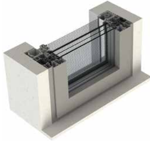
BORA TOP INCAS STANDARD 20/20
