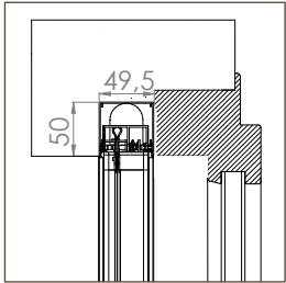
BORA INCAS SR MIDI 20
