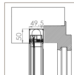
BORA INCAS MIDI 20/20
