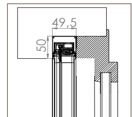
BORA TOP INCAS MIDI 35/35
