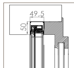
BORA TOP INCAS MIDI 50/50
