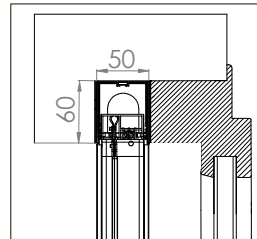
BORA TOP INCAS SR STANDARD 35
