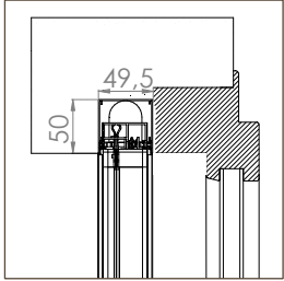
BORA INCAS SR MIDI 50
