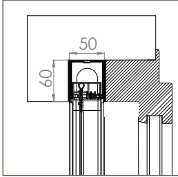
BORA INCAS SR STANDARD 50
