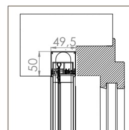
BORA INCAS MIDI 35/35
