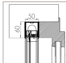
BORA TOP INCAS STANDARD 20/20
