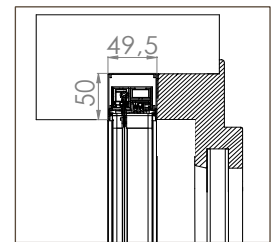
BORA TOP INCAS MIDI 20/20
