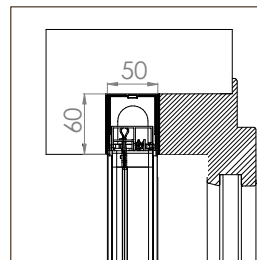
BORA INCAS STANDARD 50/50
