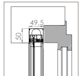
BORA INCAS MIDI 50/50
