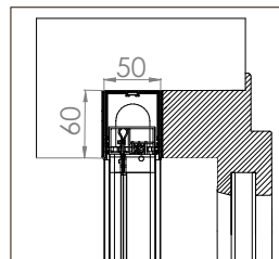
BORA TOP INCAS SR STANDARD 50
