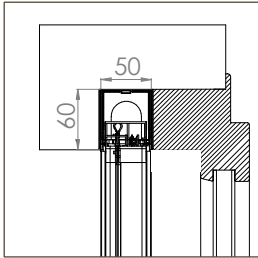
BORA INCAS SR STANDARD 20
